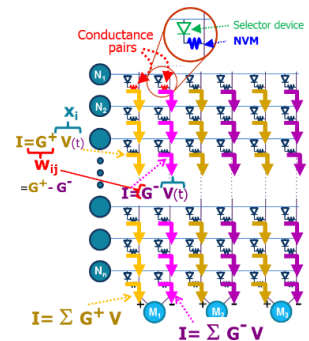
Figure 12. In-memory Computation Example (Geoffrey Burr)
